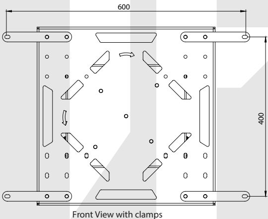
Front View with clamps
