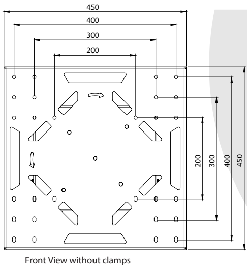
Front View without clamps
